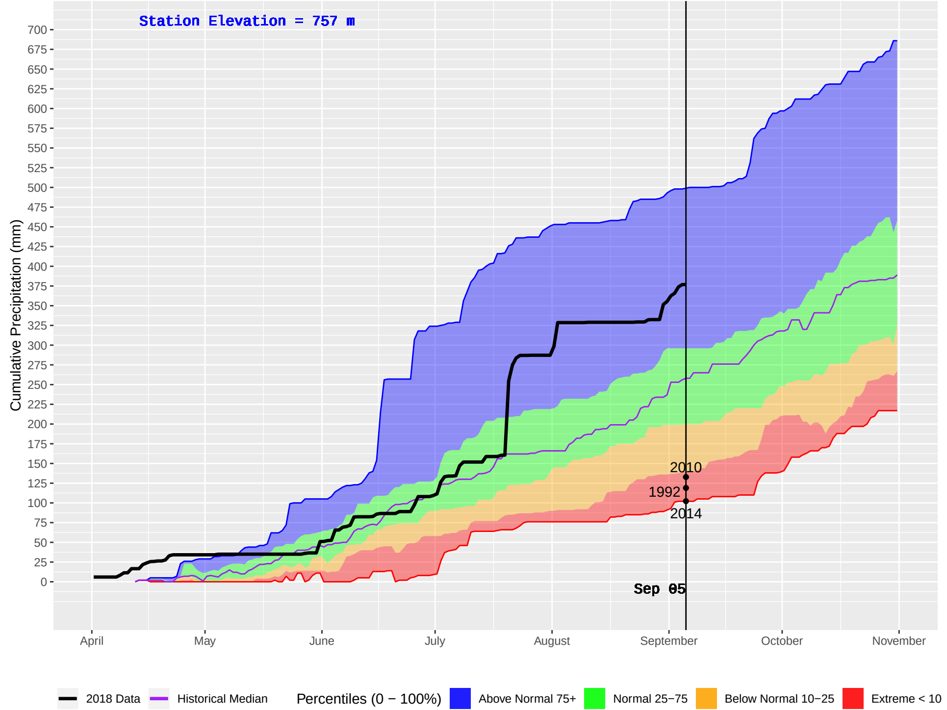
LEMORAY (140) : Historical (1988–2016) and Current (2018) Daily Cumulative Precipitation
