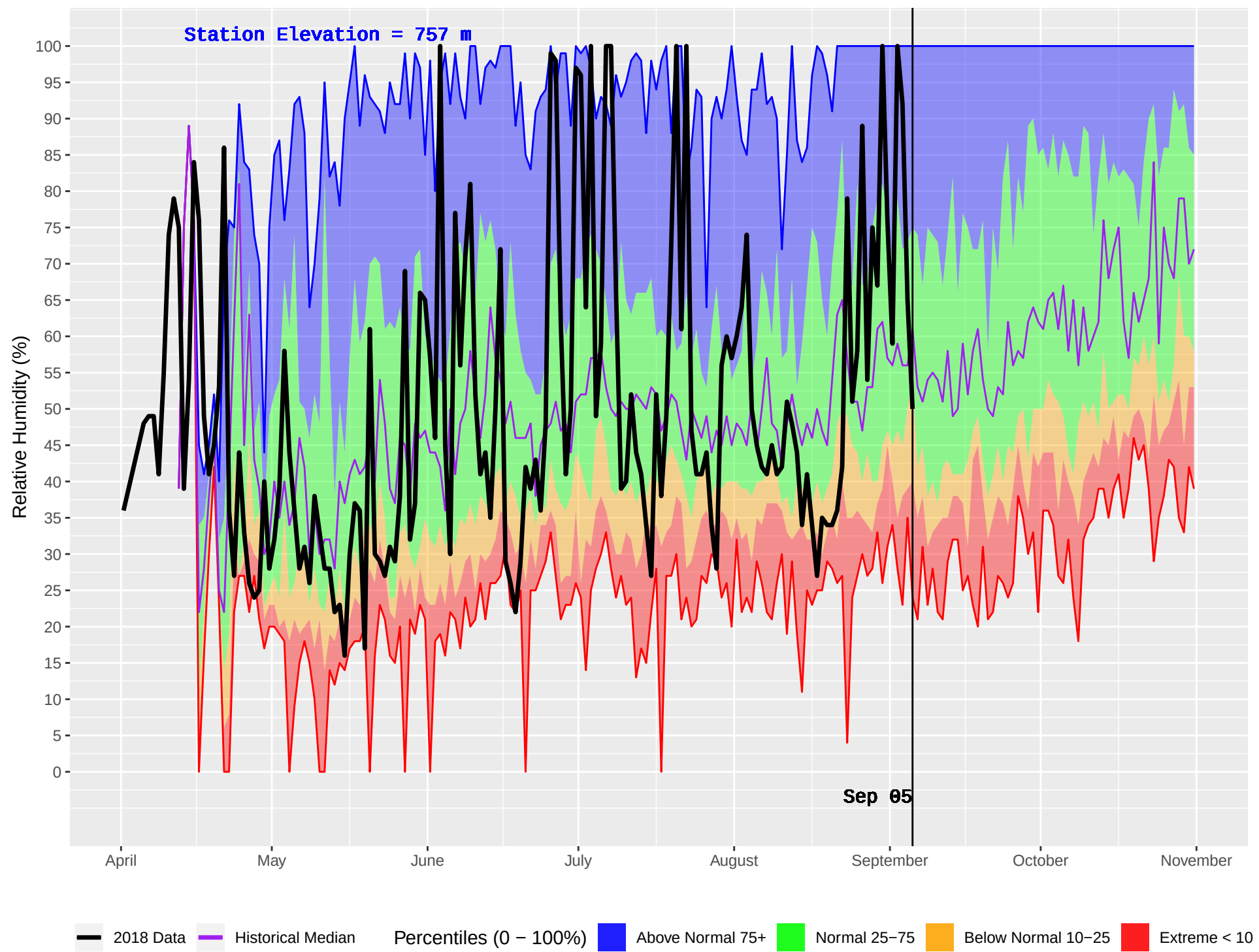
LEMORAY (140) : Historical (1988–2016) and Current (2018) Daily Relative Humidity
