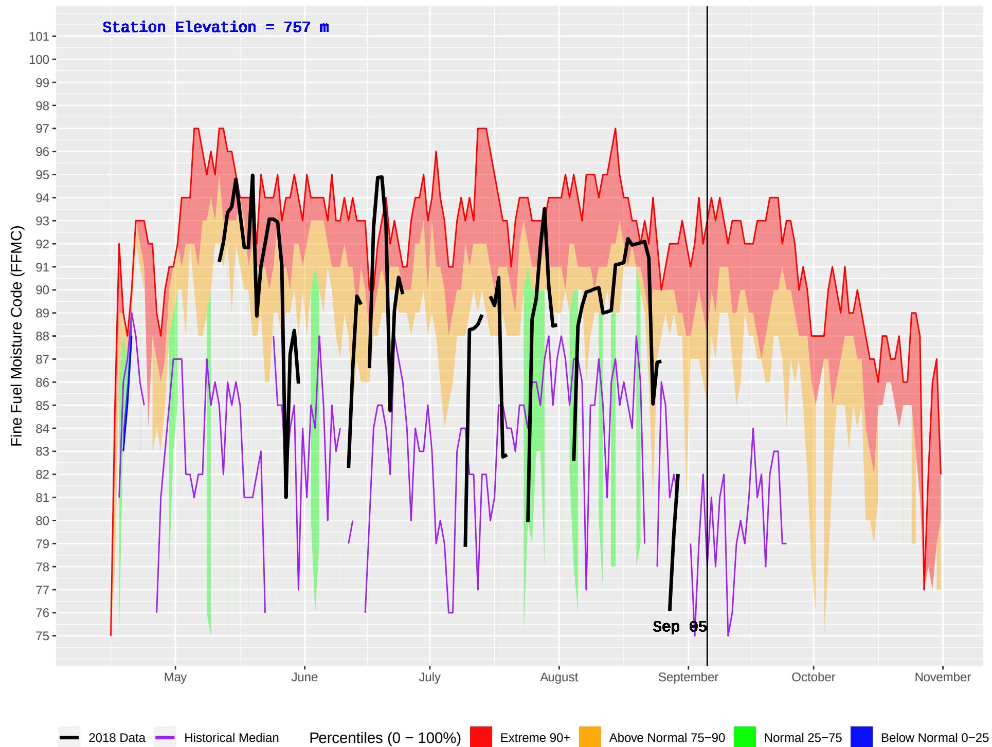
LEMORAY (140) : Historical (1988–2016) and Current (2018) Daily Fine Fuel Moisture Code (FFMC)
